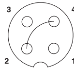
Pin assignment M12 socket, 3-pos., PIN 2+4 bridged, A-coded, view female Pin assignment M12, 3-pos. side
